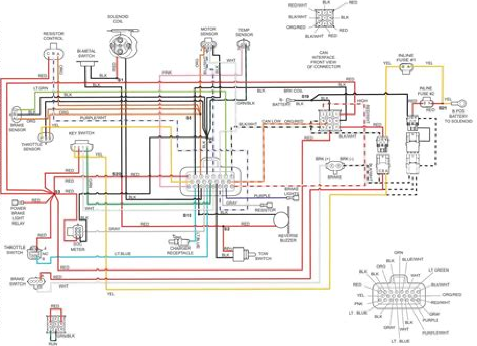
FIG. 30 Main Wiring Harness Diagram (6 December 2009 through 23 January 2012)
