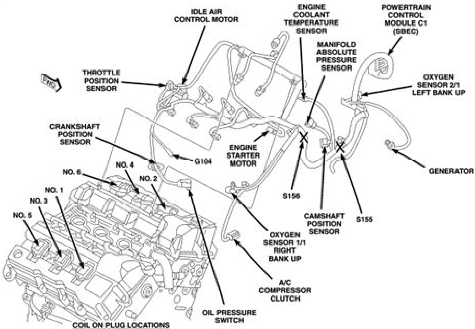
ENGINE CONNECTORS 2.7L
