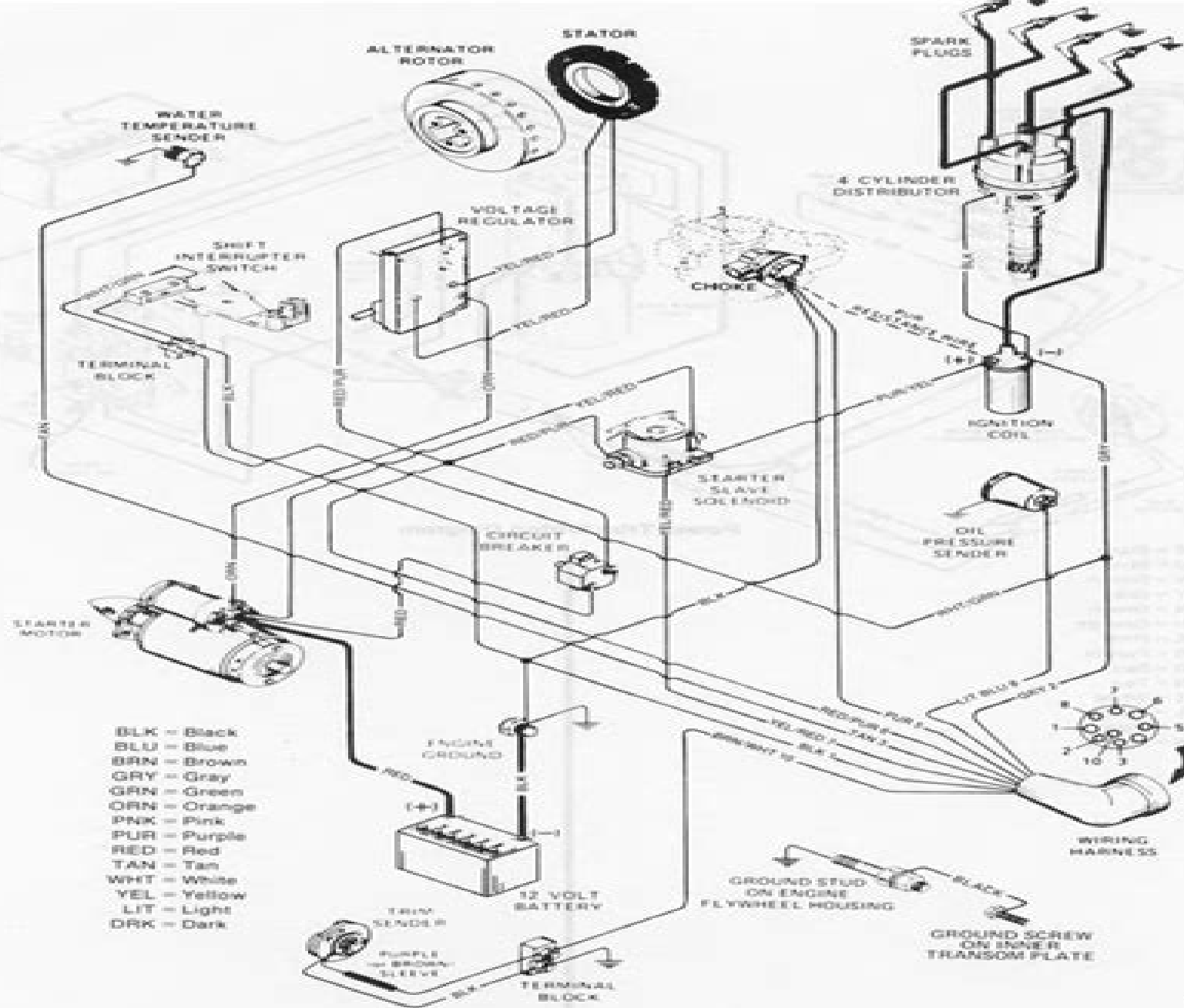
Engine Electrical System Wiring Diagram
