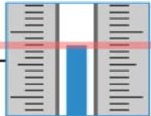
Judgment uncertainty
