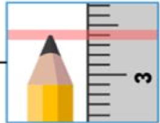
Judgment uncertainty
