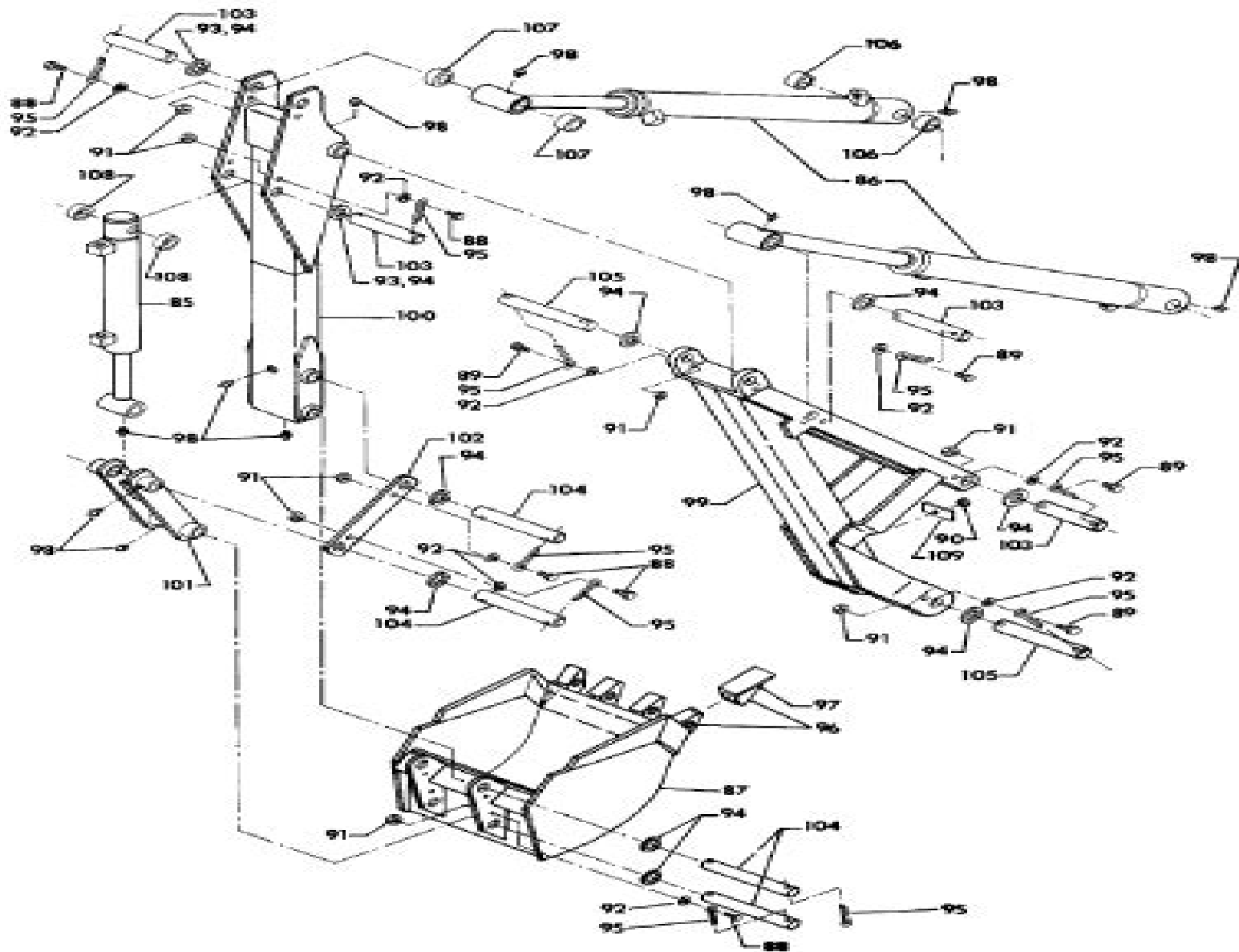
KUBOTA TRACTOR B670 BACKHOE Figure: 17 - BACKHOE - BOOM, DIPPERSTICK, AND BUCKET
