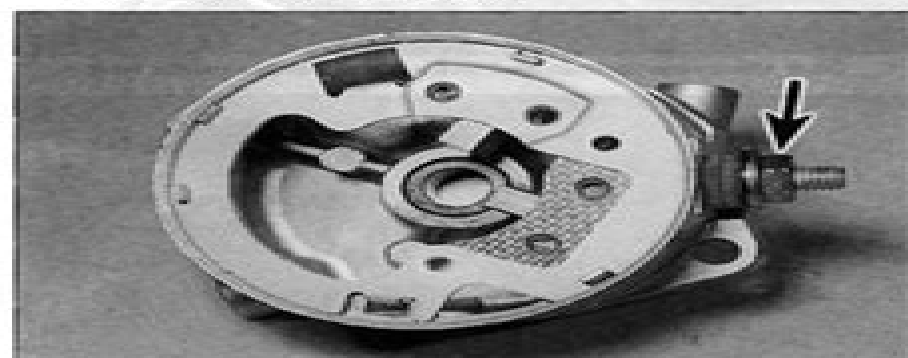
31.5a Unscrew the nut (arrowed) and remove the washers . . .
