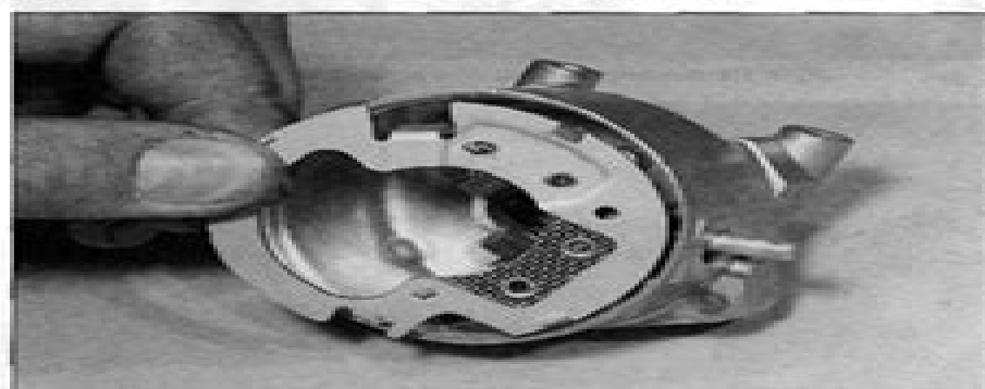
31.5b . . . then remove the brushplate assembly
