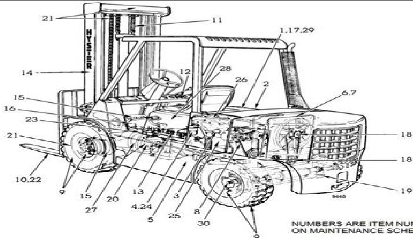
FIGURE 1. MAINTENANCE POINTS
