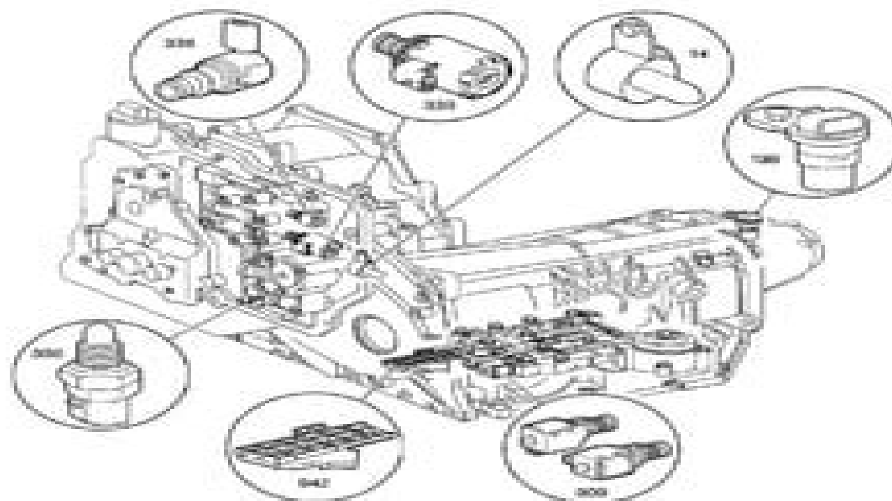
Fig. 17: Automatic Transmission Electronic Component Views Courtesy of GENERAL MOTORS CORP.
