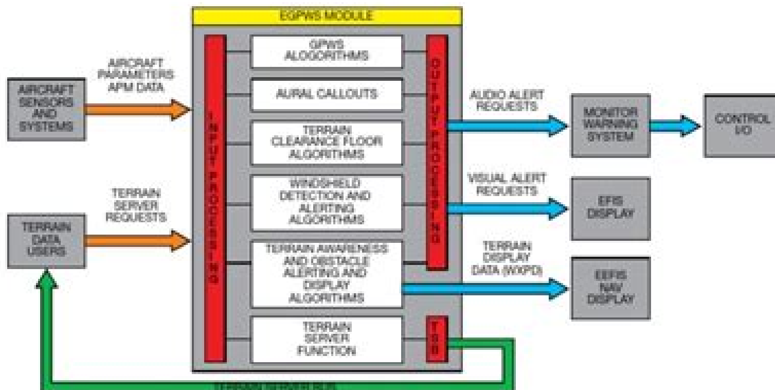
Figure 34-102. Enhanced Ground Proximity System
