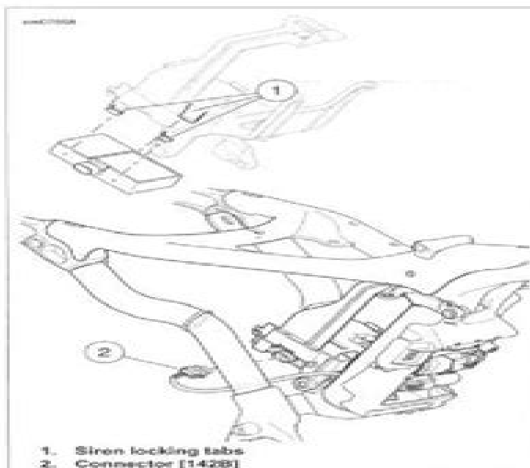
Figure 6-13. Smart Siren
