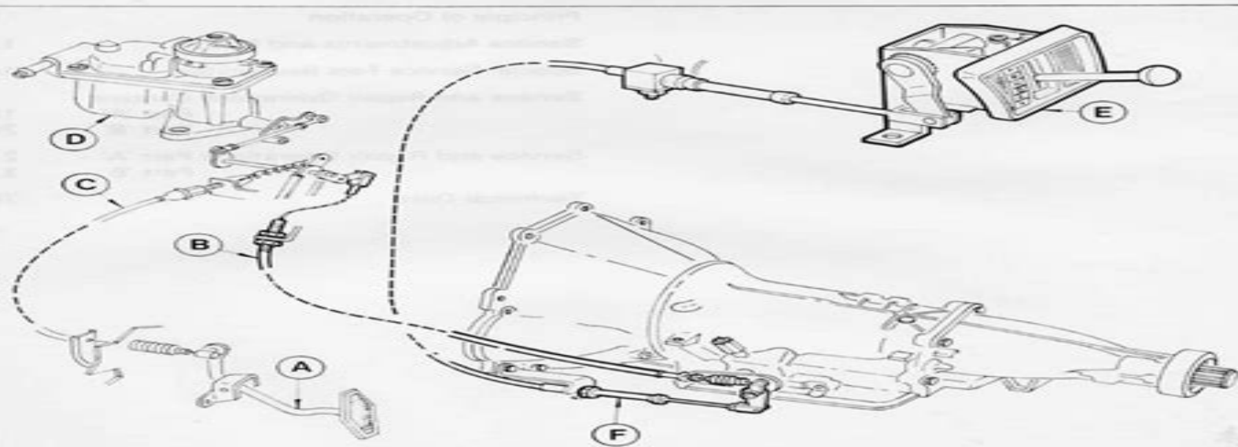
Fig. 1. Automatic transmission operating system
