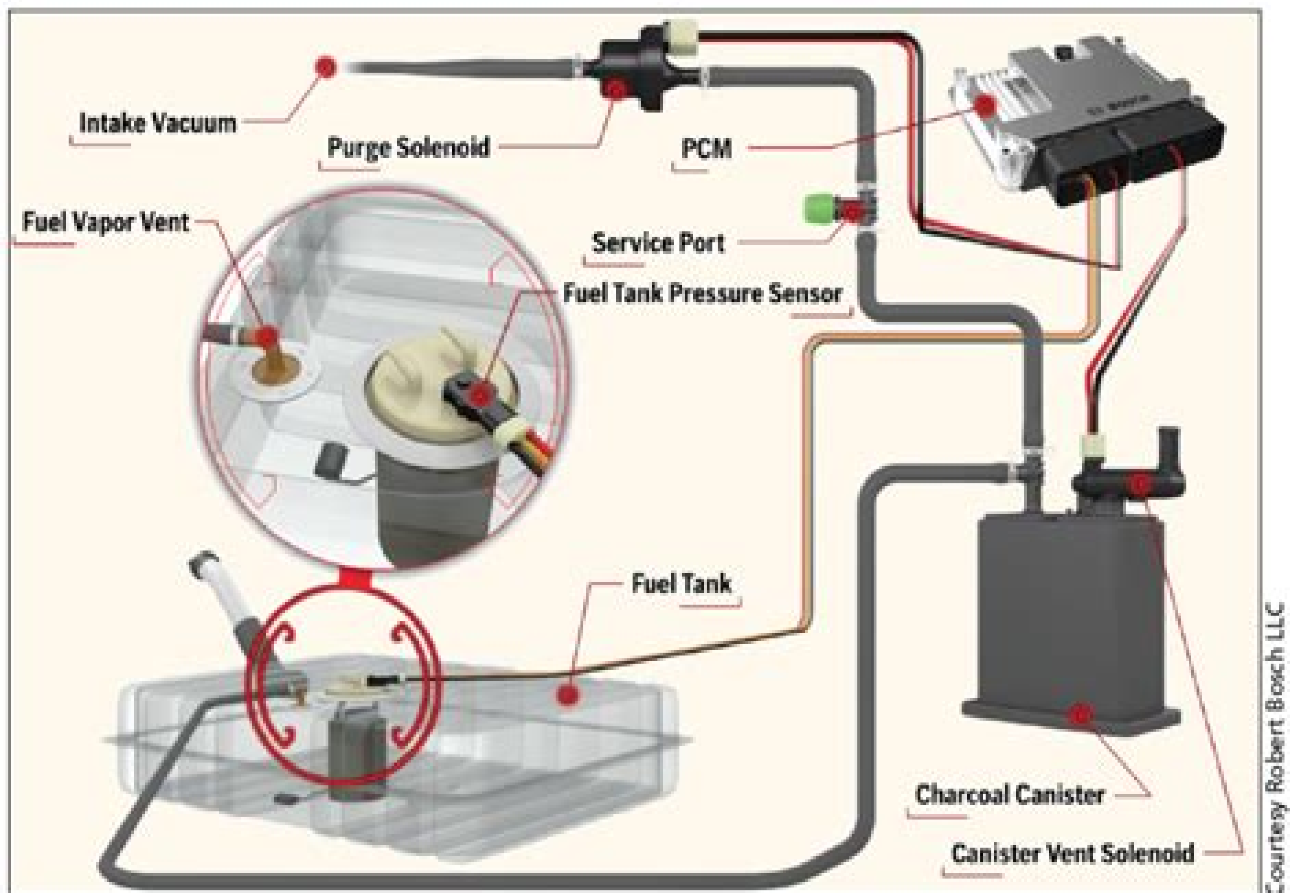
Fig. 1 This illustration shows the typical layout of components associated with Ford's vacuum-based evaporative emissions system, which has been in use for many years.
