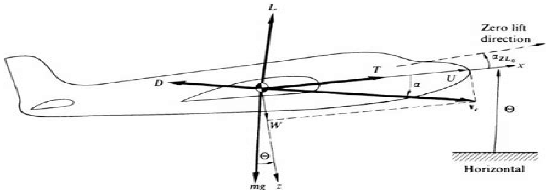
Fig. 3.5. Flight vehicle in a condition of perturbed longitudinal motion.
