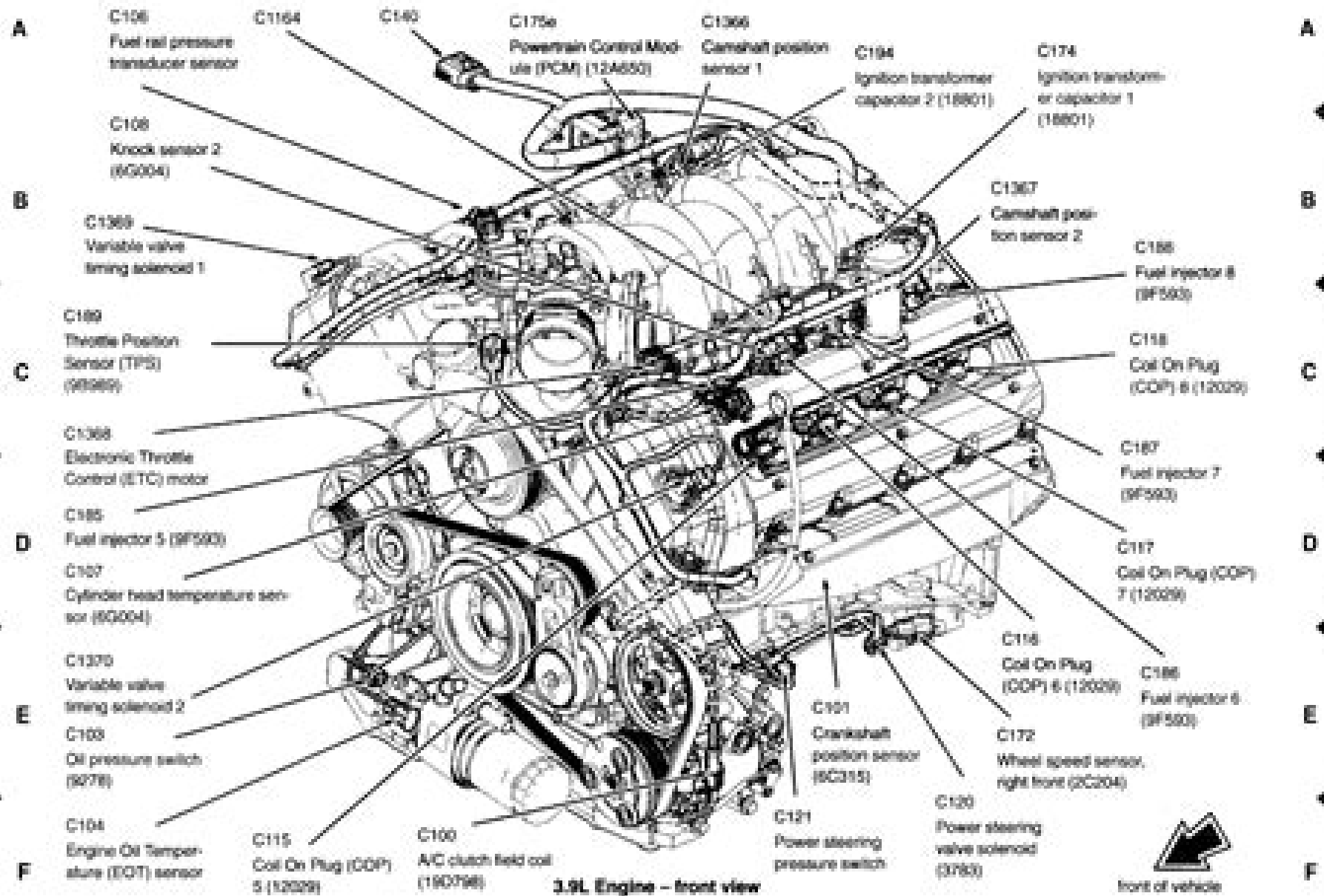
3.9L Engine - front view
