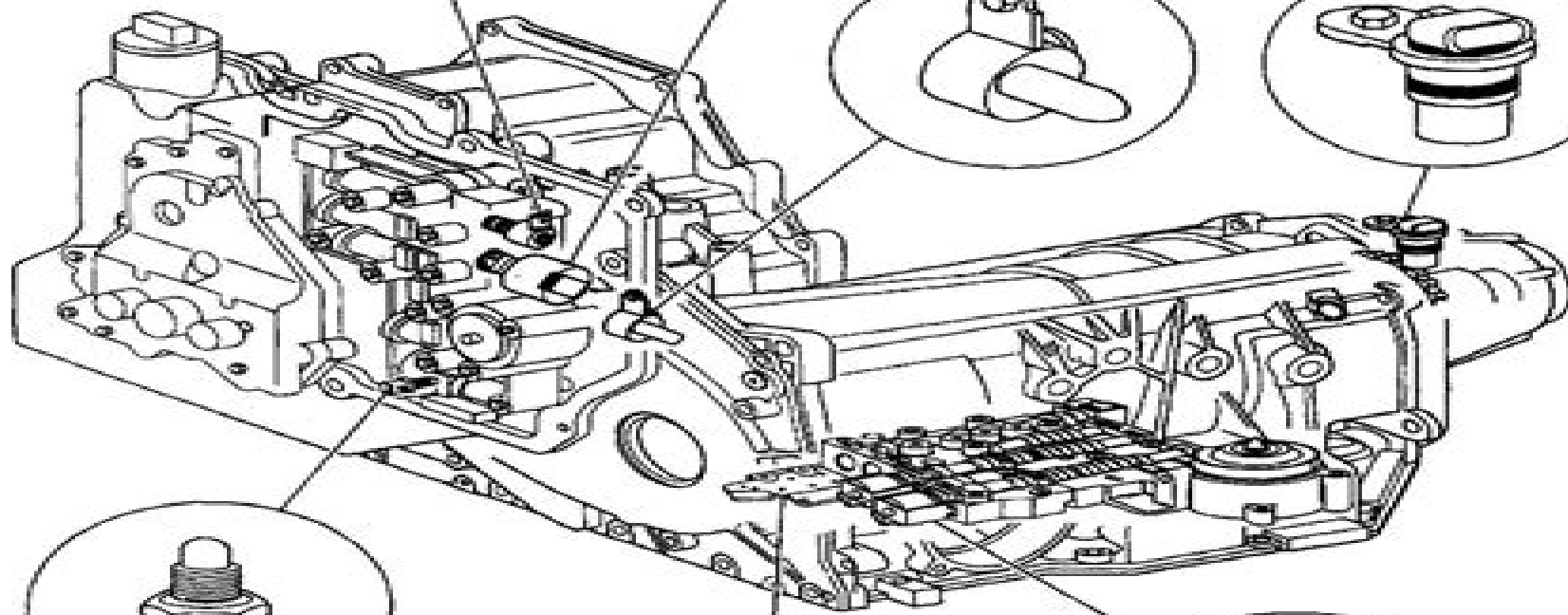
TRANSAXLE INPUT SPEED SENSOR
