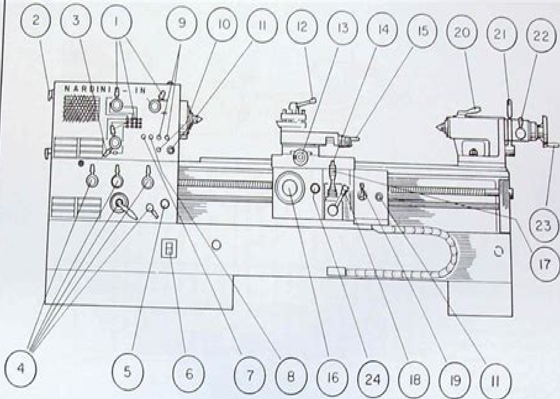
FIG. 5 LATHE CONTROLS
