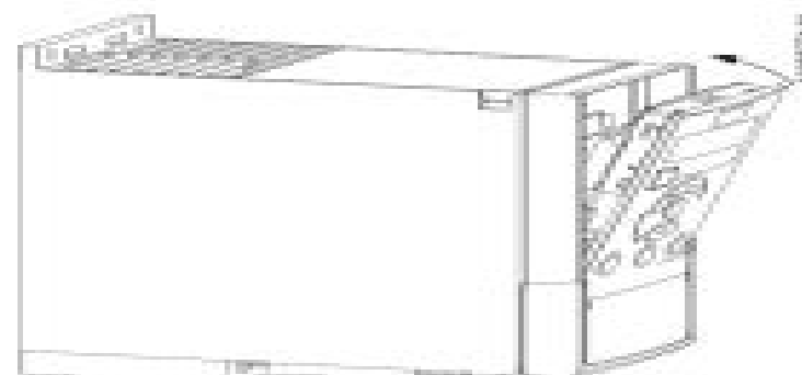
Illustration 1.2 Push the Top of the LCP into Place
