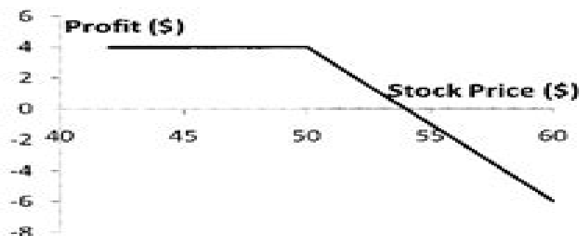
Figure S9.2 Investor's profit in Problem 9.2
