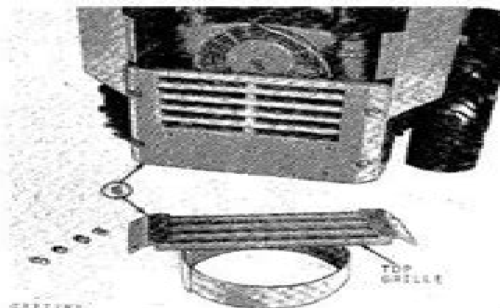
Fig. 3-Removing Upper and Lower Grilles
