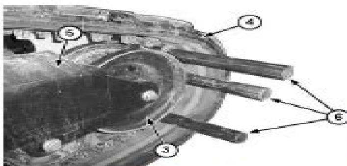
CTL Track Removal
