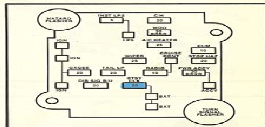
Fig. 8A-71 — Fuse Panel
