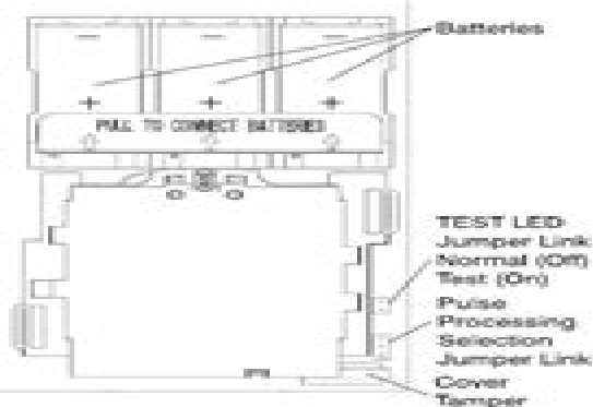
Figure 4. Printed Circuit Board (PCB)
