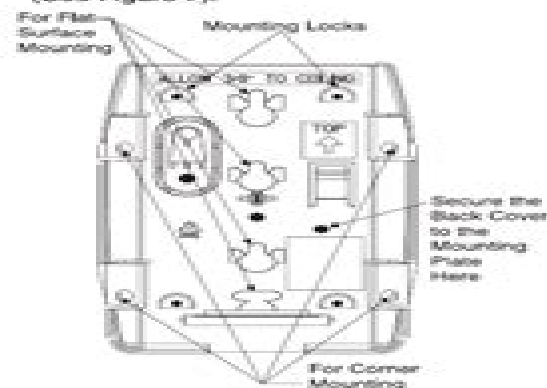
Figure 7. Mounting Plate
