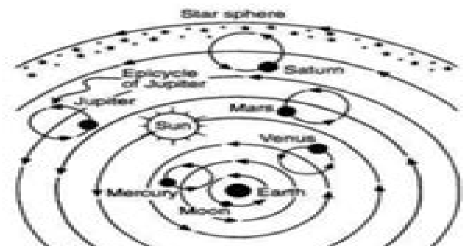
Geocentric model
