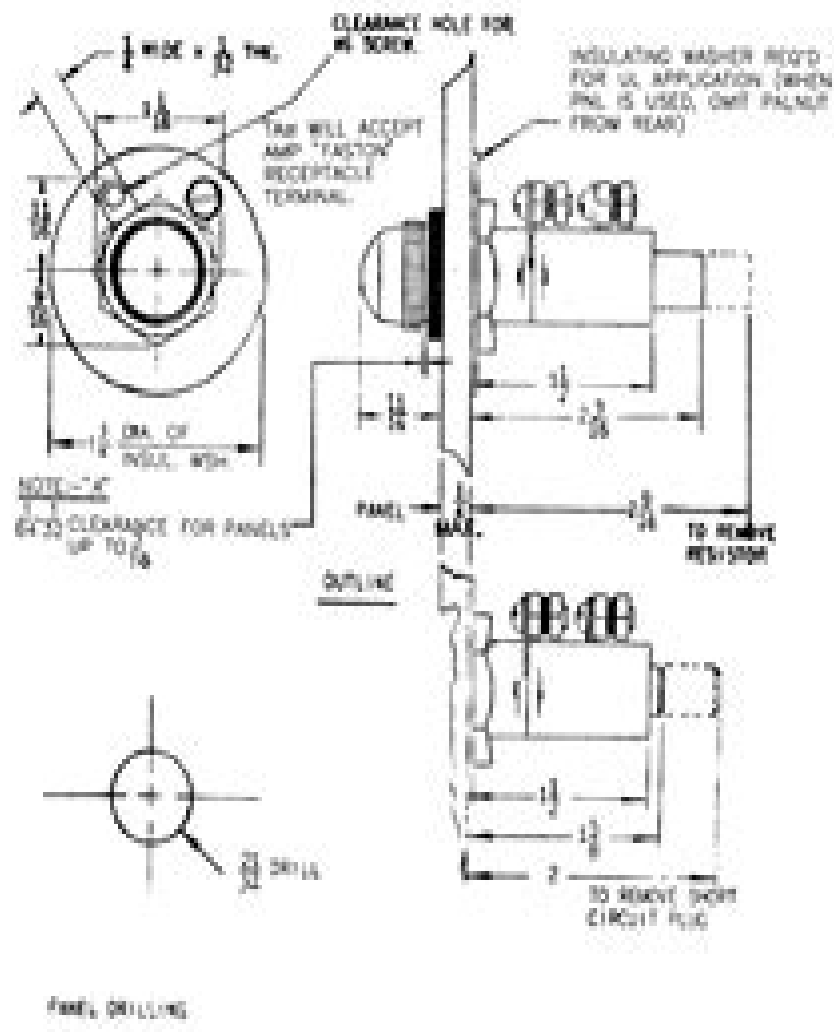
Figure 4 illustrates the outline and panel drilling for holes indicating lamp type ET-12.
