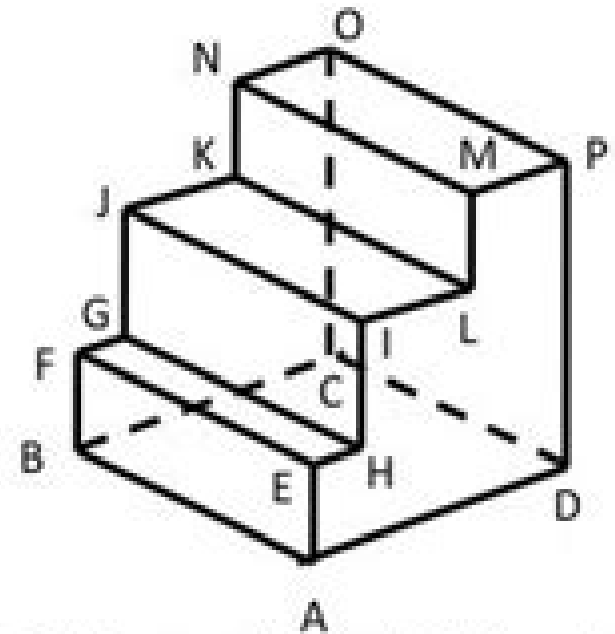
Fig 13b Isometric View (Hidden details)
