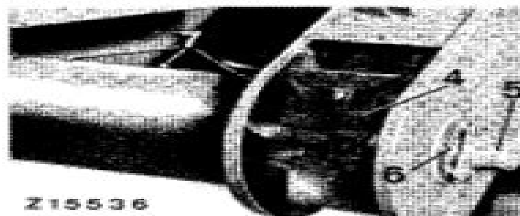
Fig. 22 — Tailings Elevator, Lower Section (975 Shown)
