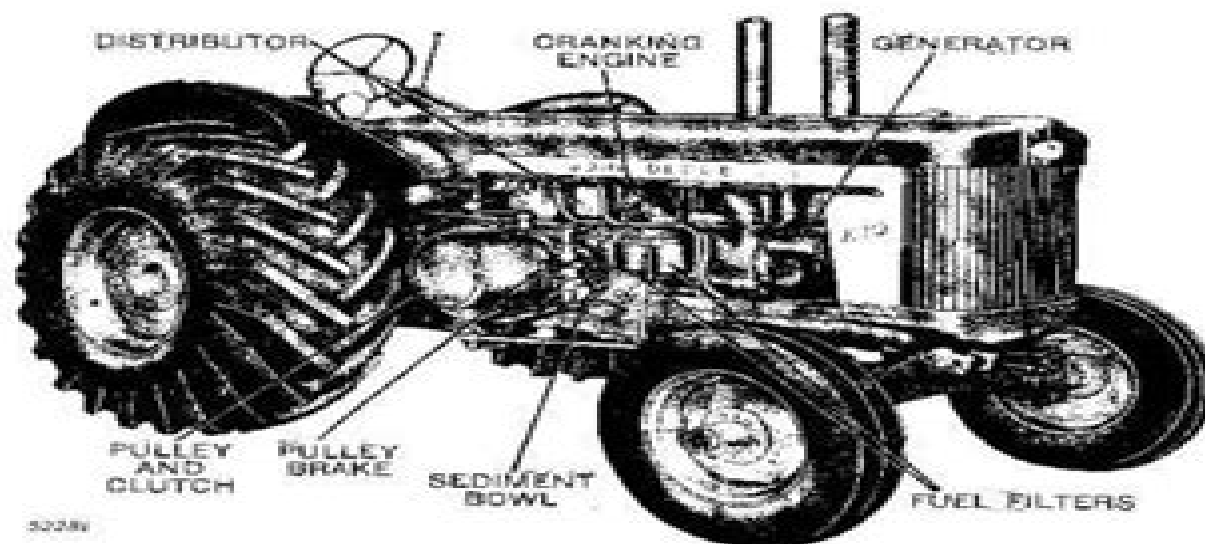
Figure 10-5-1—John Deere "820" Series Diesel Tractor—Pulley Side
