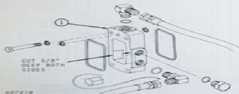
Fig. 1A-Auxiliary Outlet Coupler Kit
