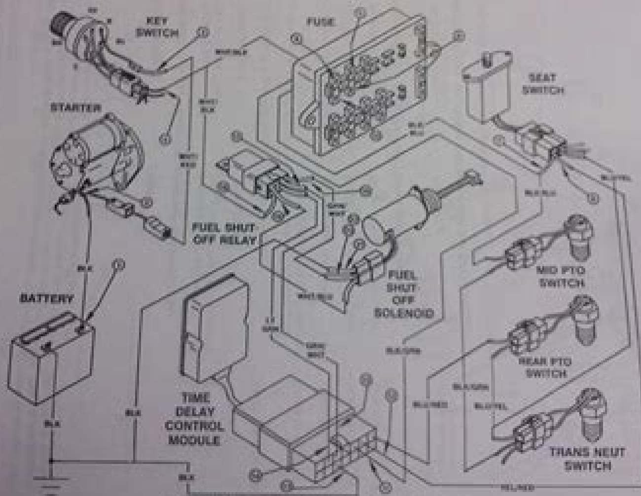
FUEL SHUT-OFF PULL-IN SYSTEM TEST POINTS (NEW VERSION)
