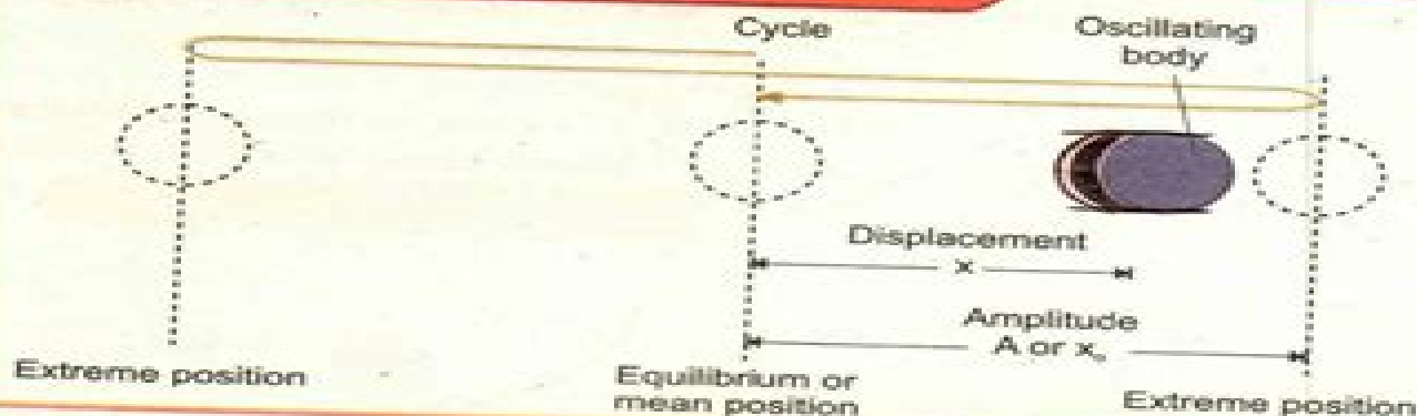
Figure 10.1 - Terminologies of Oscillatory Motion
