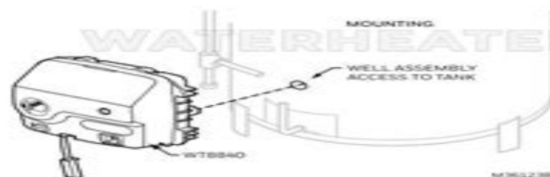
Fig. 2. Mounting the WT88xx controls on the water heater tank.
