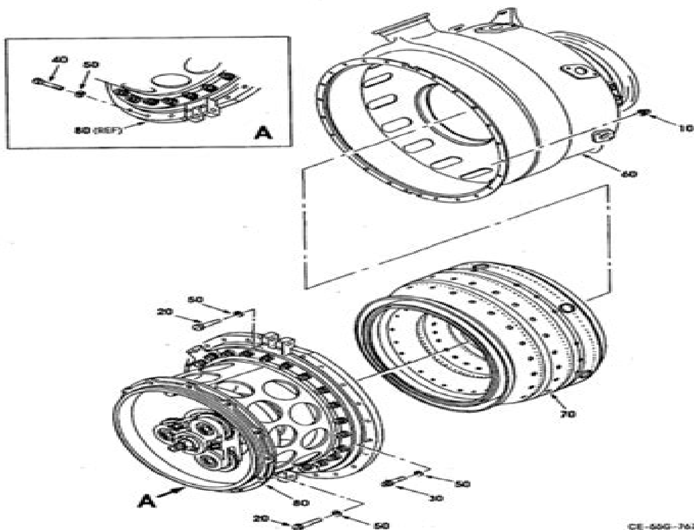
Hot Section Components (Partial Breakdown) Figure 601
