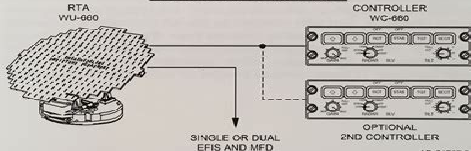
PRIMUS® 660 Configurations Figure 2-1
