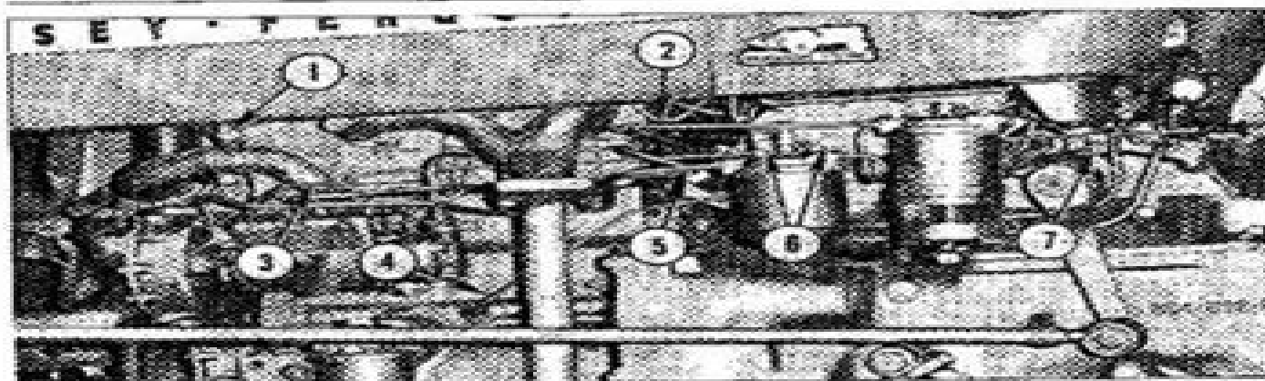
Fig. 10 - Left Hand Side View of Diesel Engine
