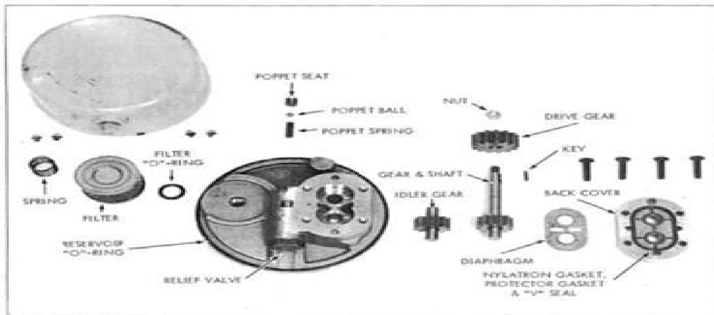
Fig. 4 - Disassembled View of Steering Pump - MF 150 - Diesel
