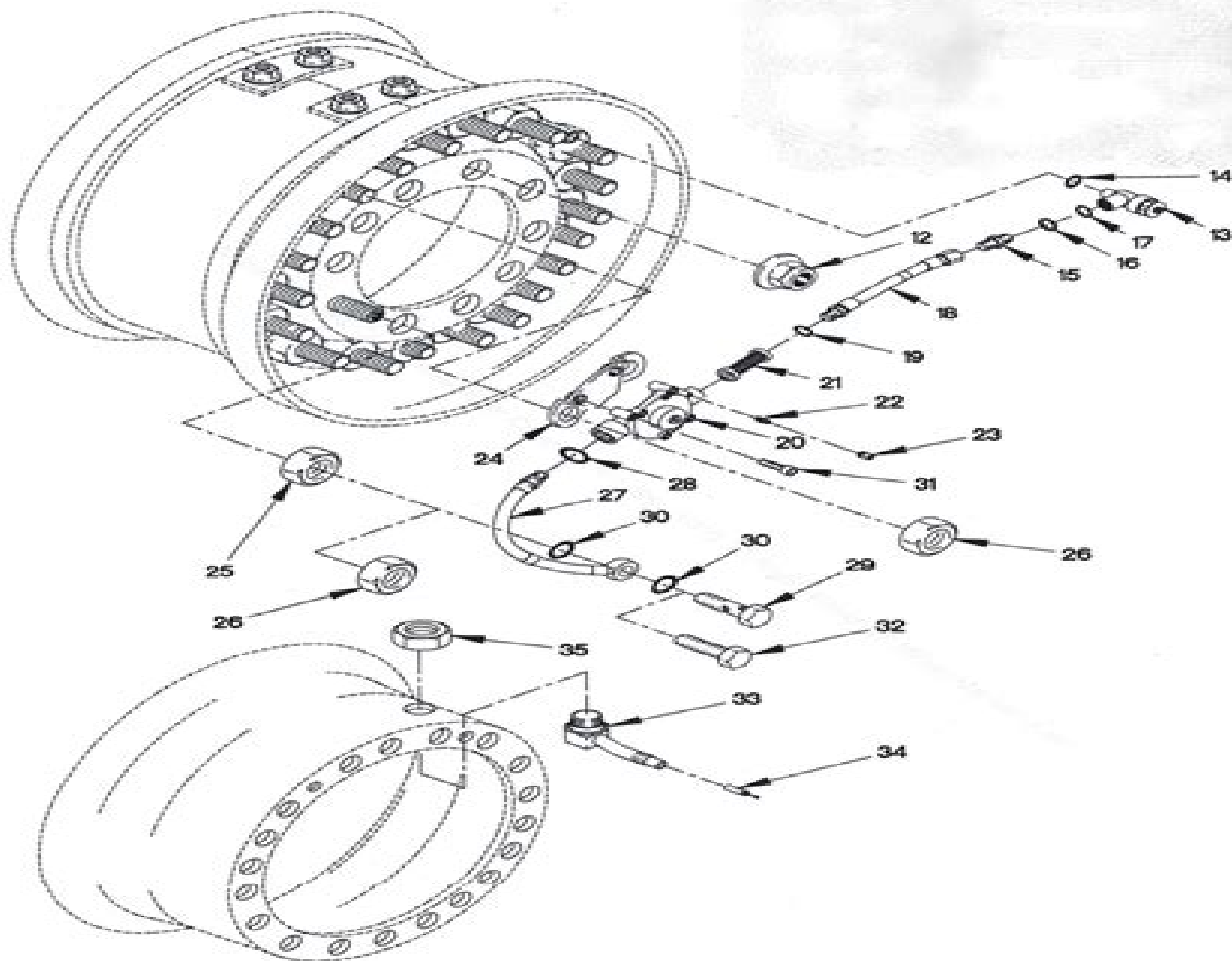
FIGURE 158. WHEEL ASSEMBLY AND CTIS VALVE (SHEET 2 OF 2)
