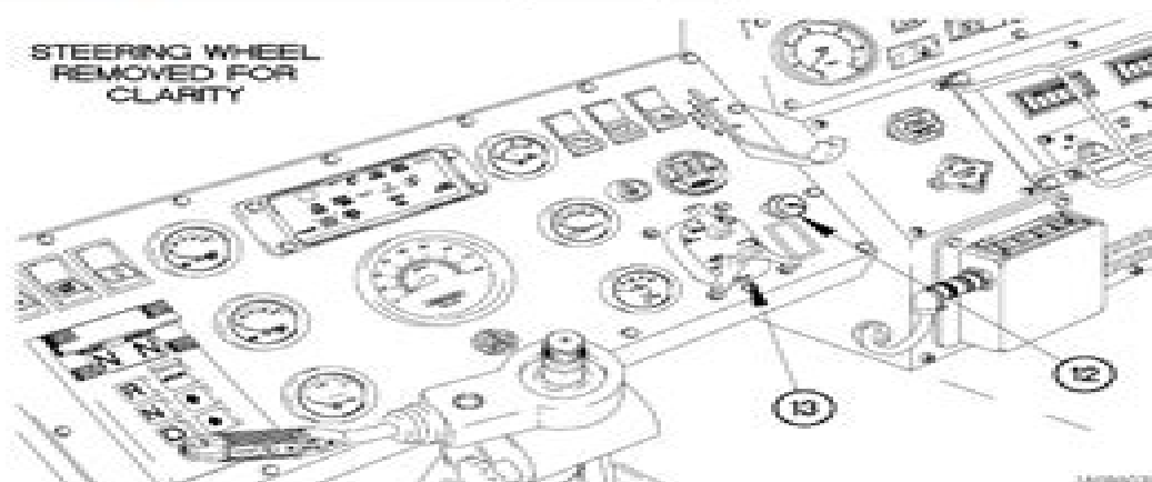
Figure 1-13. Electrical System (Cont)
