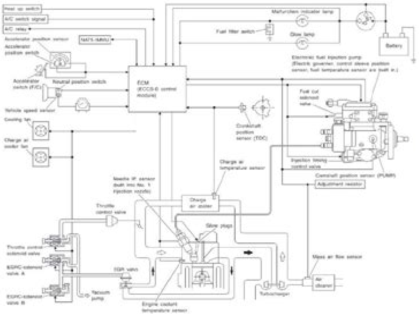
System Diagram
