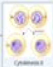
Cytokinesis II
