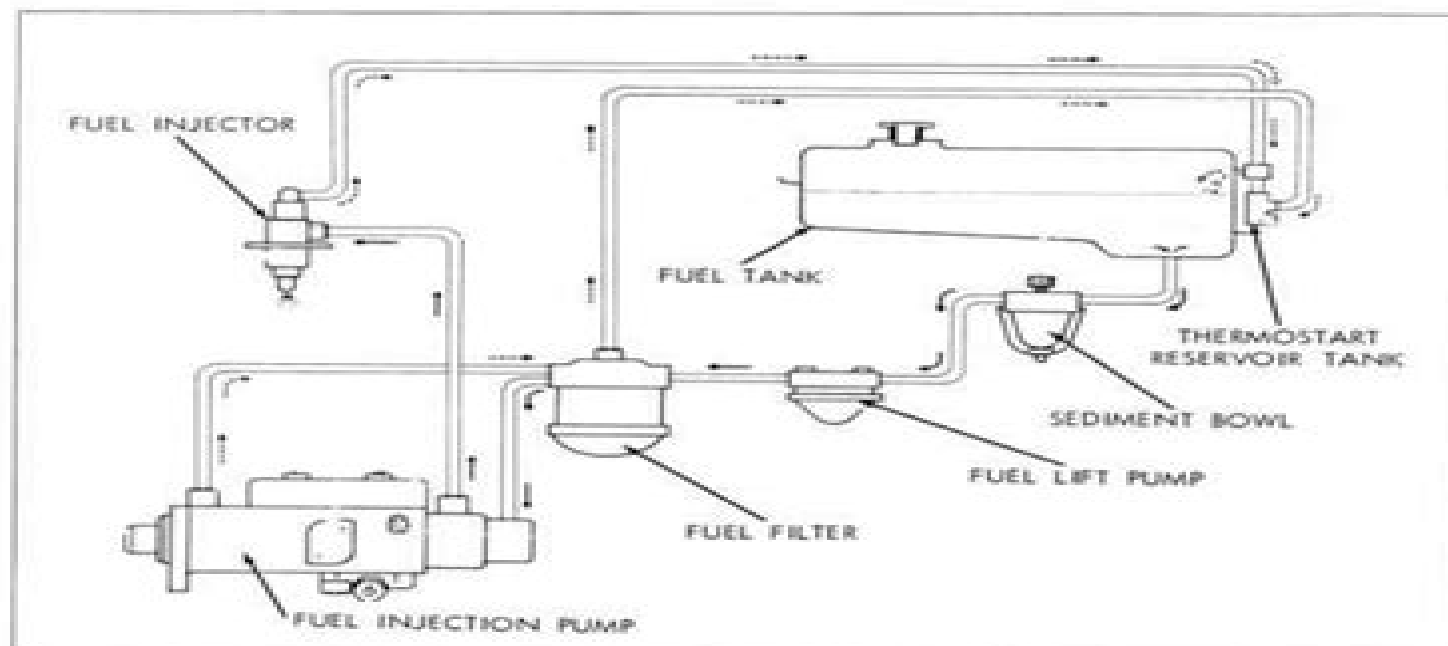
Fig. 1 - Fuel System of A4.10P Engine
