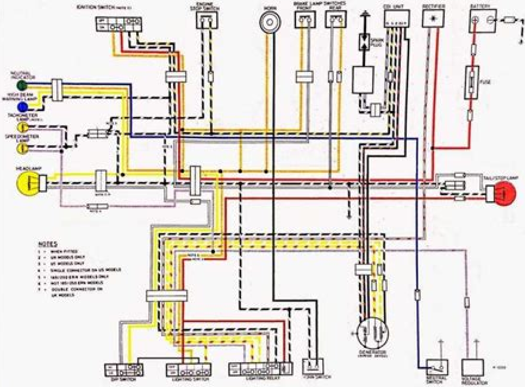
Wiring diagram - TS 250
