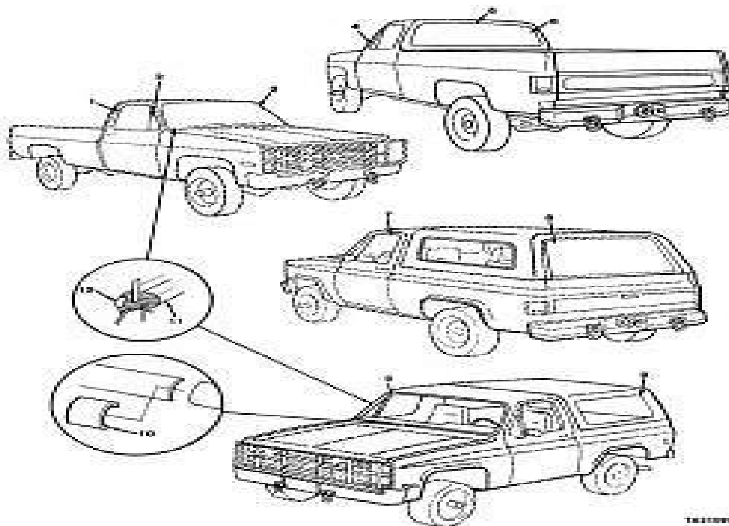
FIGURE 180. WINDSHIELD AND WINDOW GLASS.
