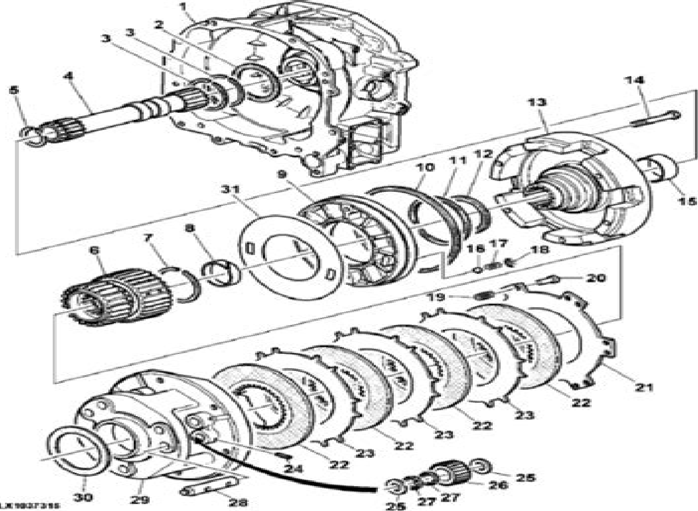
LX1047315-UN: Forward clutch with planetary drive
