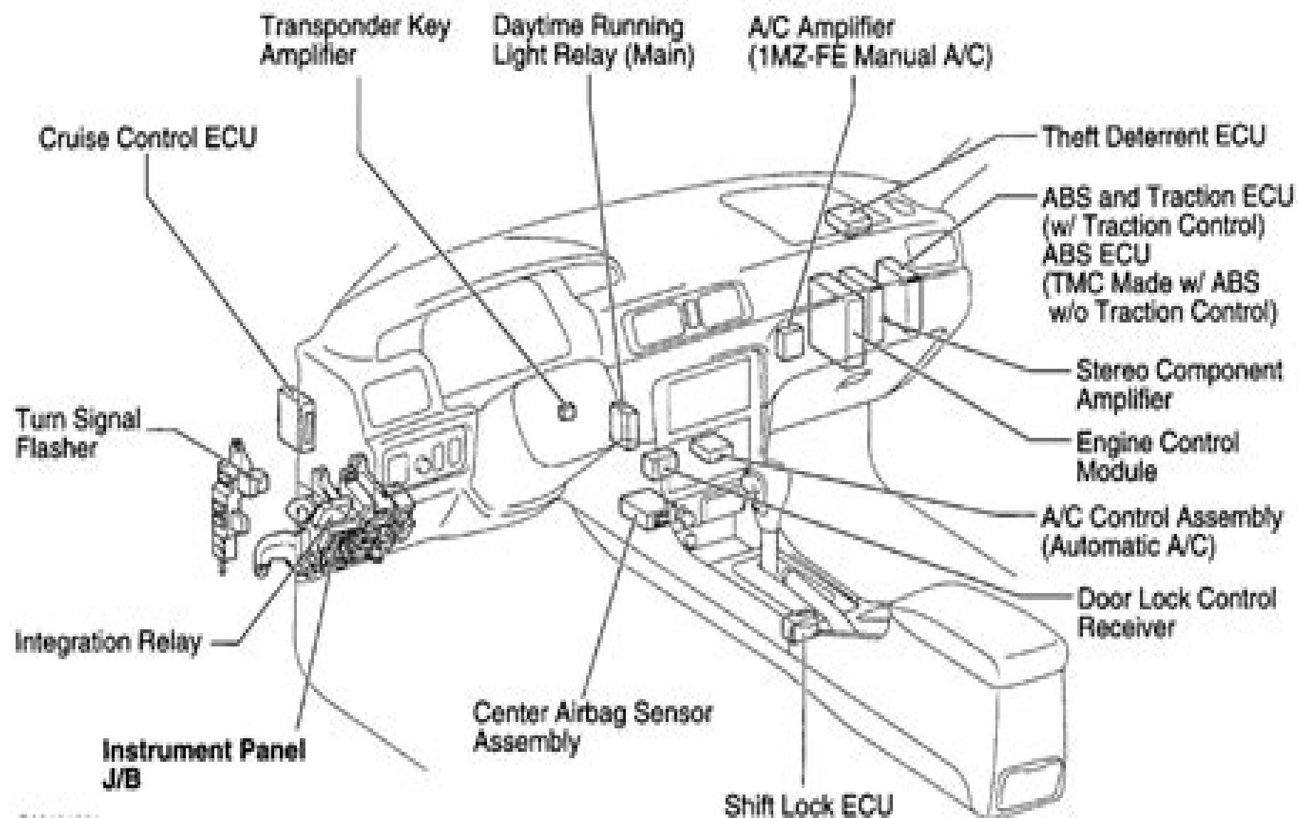
Fig 1: Locating Instrument Panel Electrical Components
