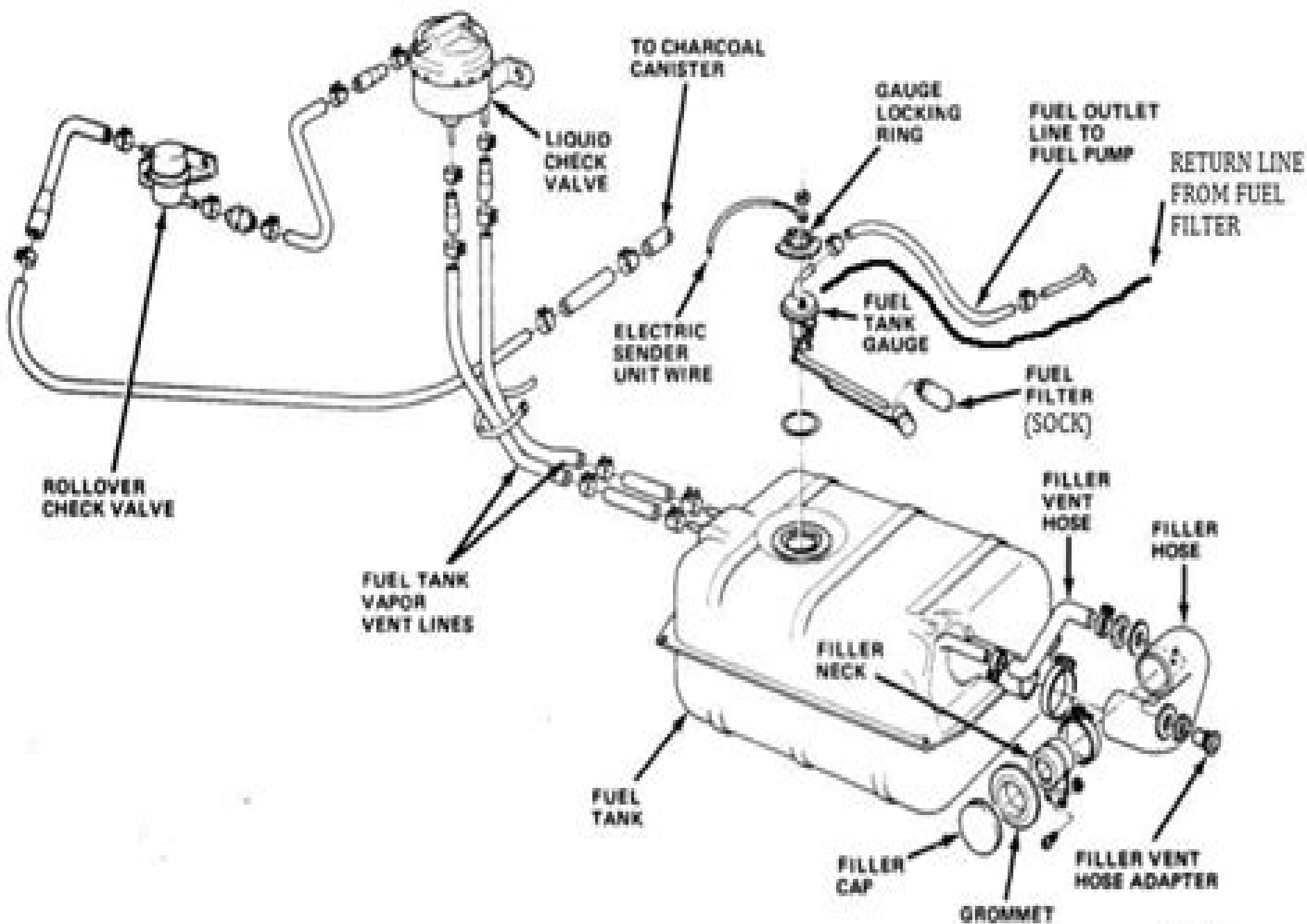
Fig. 4-4 Fuel Tank and Vent Lines—CJ-5 and CJ-7
