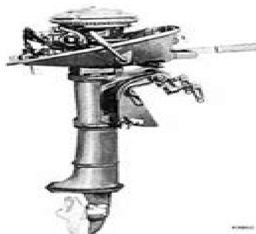
Figure 2-2. Starboard Side, Standard Gearcase
