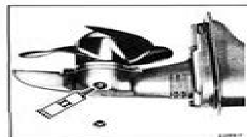
Figure 2-6. Standard Gearcase
