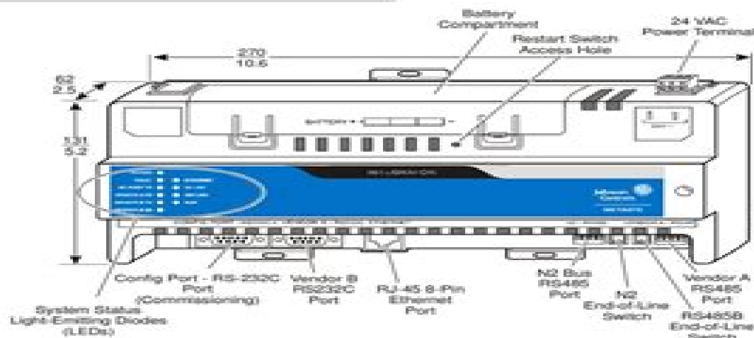
Figure 1: Front of MIG3500 Showing Dimensions, mm (in.), and Physical Features
