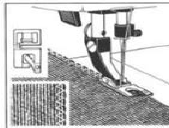
411 85 24-01. Presser foot for 2 mm rolled hem. For medium zig-zag stitching, stitch length 3. Suitable for light fabrics.
