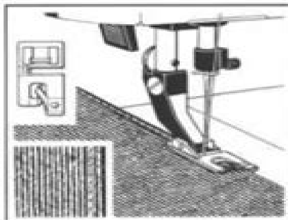
411 85 22-01. Presser foot for 2 mm hemming. For straight stitching or small zig-zag stitching, stitch length 1.5.
