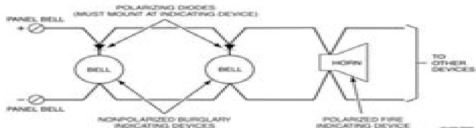
Figure 3-7: Wiring Nonpolarized Burglary Devices
