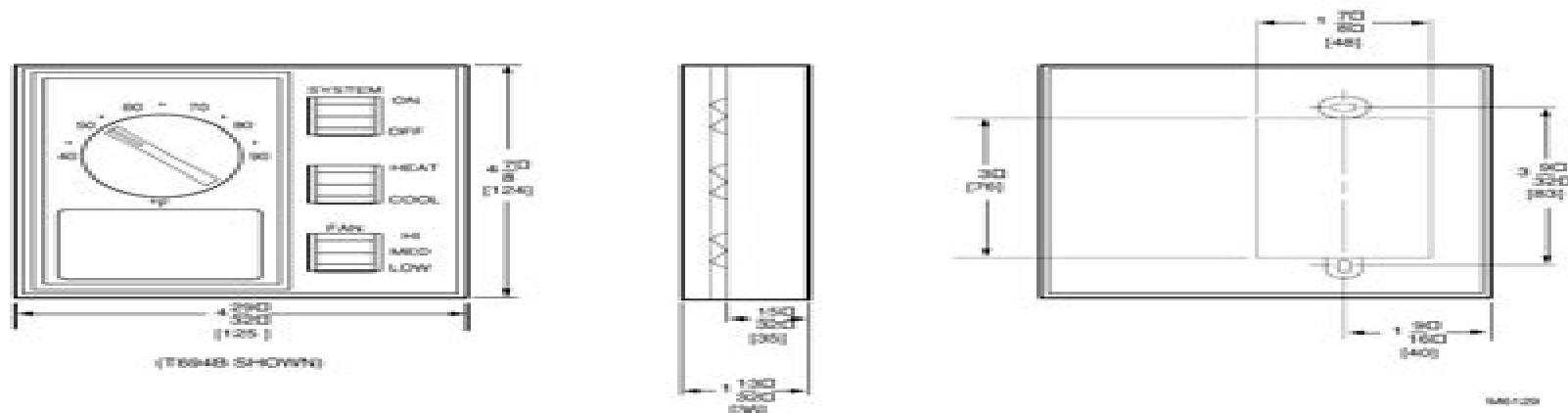
Fig. 2—T694A,B,D,F mounting dimensions in in. [mm].
